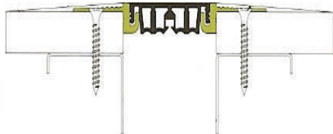
Wall systems with colorable seals
