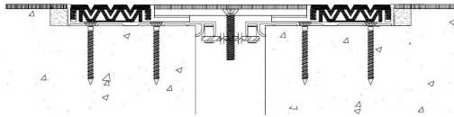
Flush Floor with colorable seals
